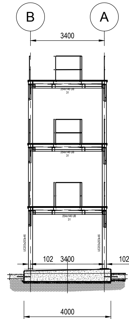
Section through Reefer Gantry Structure [1:100]
