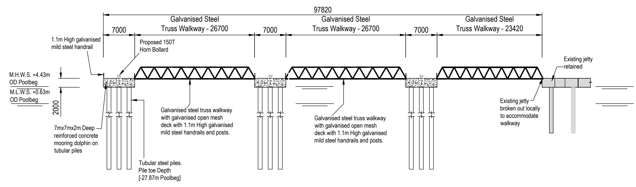
Elevation through Proposed Mooring Dolphins [1:500]
